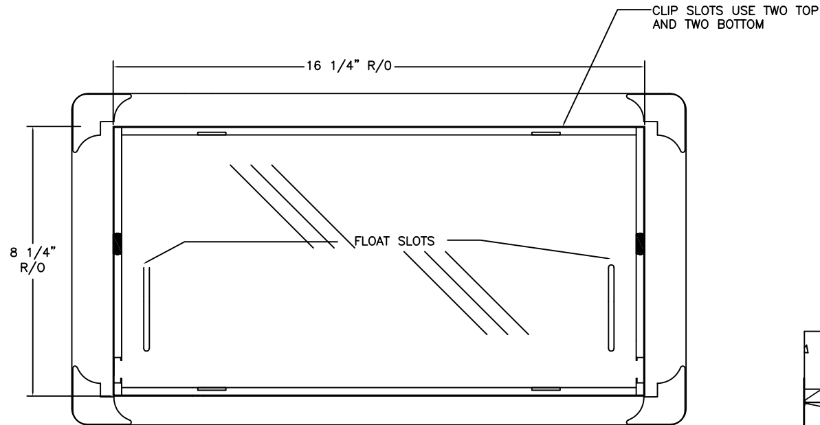
FIGURE 1 FRONT VIEW
