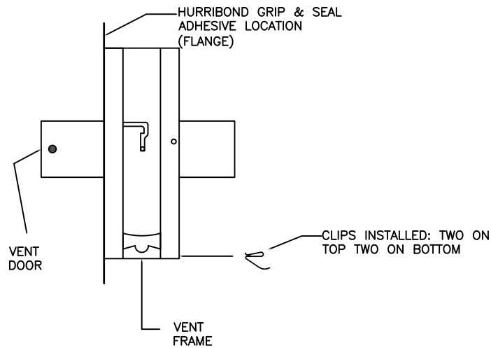
FIGURE 2 SIDE VIEW
